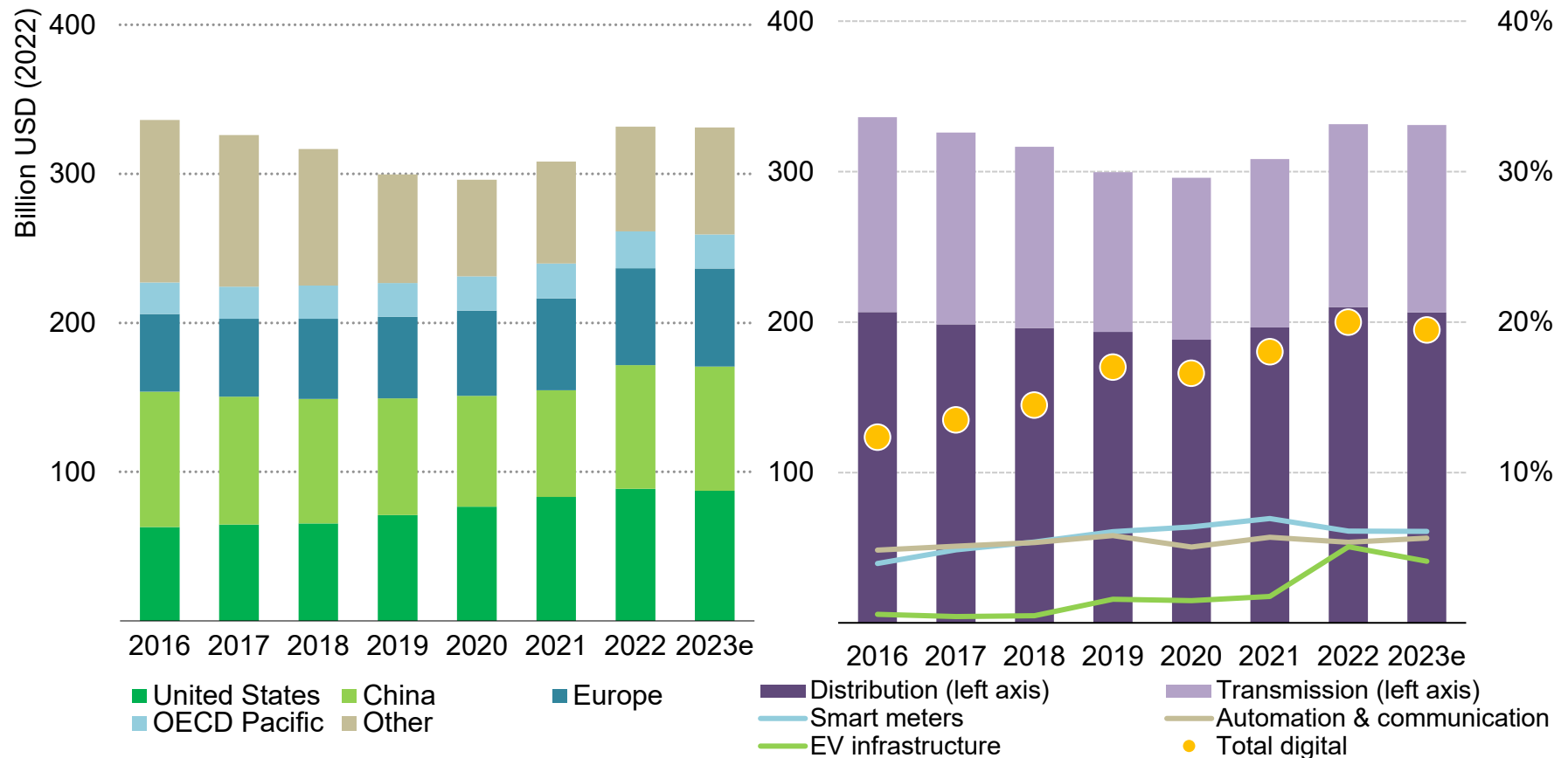
Investment in power grid infrastructure by geography (left) and segment (right), 2016-2023e
