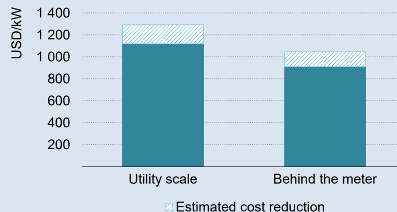
Estimated impact of the US Inflation Reduction Act on average US capital costs for battery storage (in 2022 costs)
